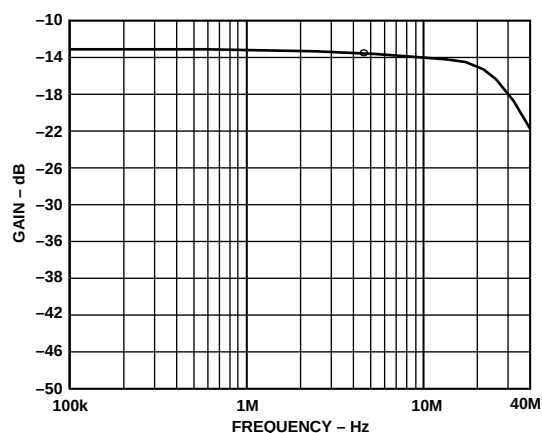
Figure 12. Frequency Response (Magnitude) of the ADG466, V_{DD}/V_{SS} = \pm 15 V and Input Signal Level of \pm 100 mV
