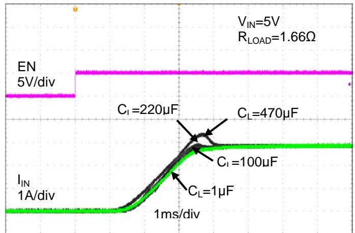
Inrush Current
