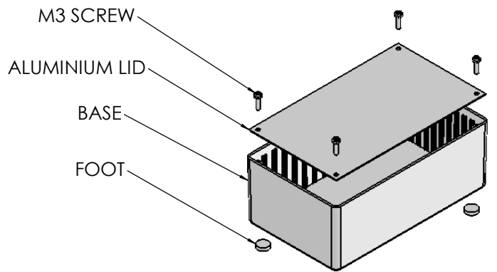
ISO VIEW 1:4
