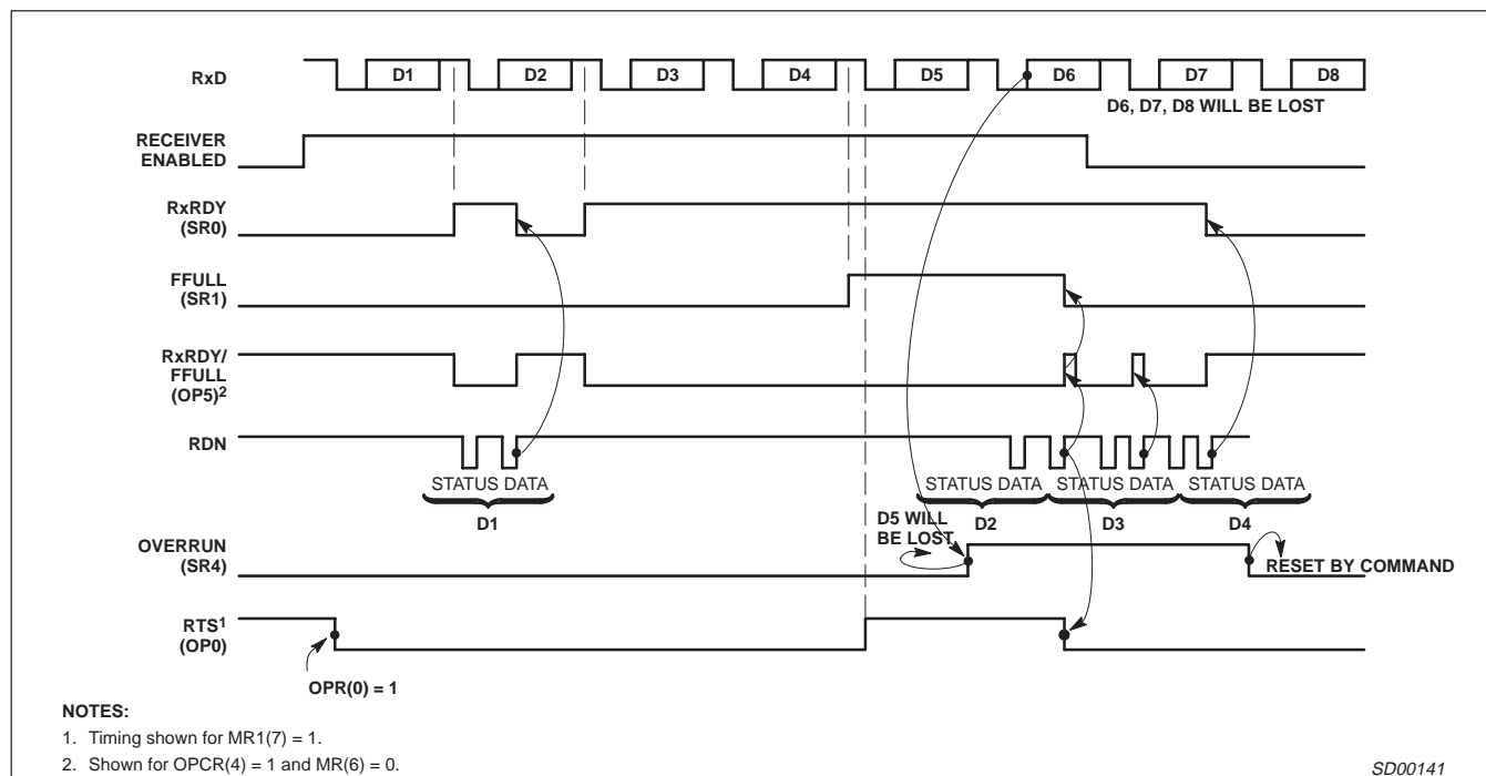
Figure 11. Receiver Timing
