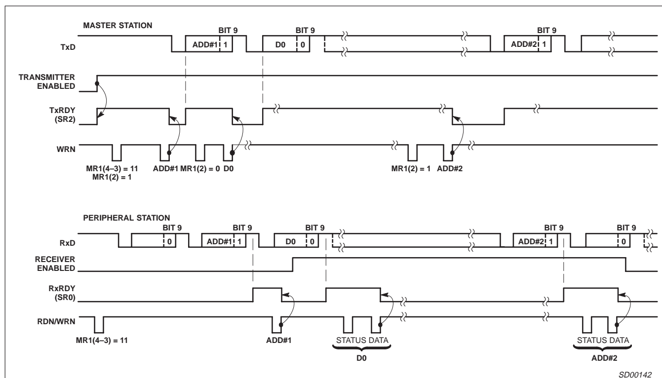
Figure 12. Wake-Up Mode
