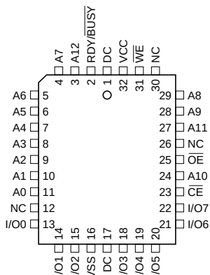
PLCC Top View
