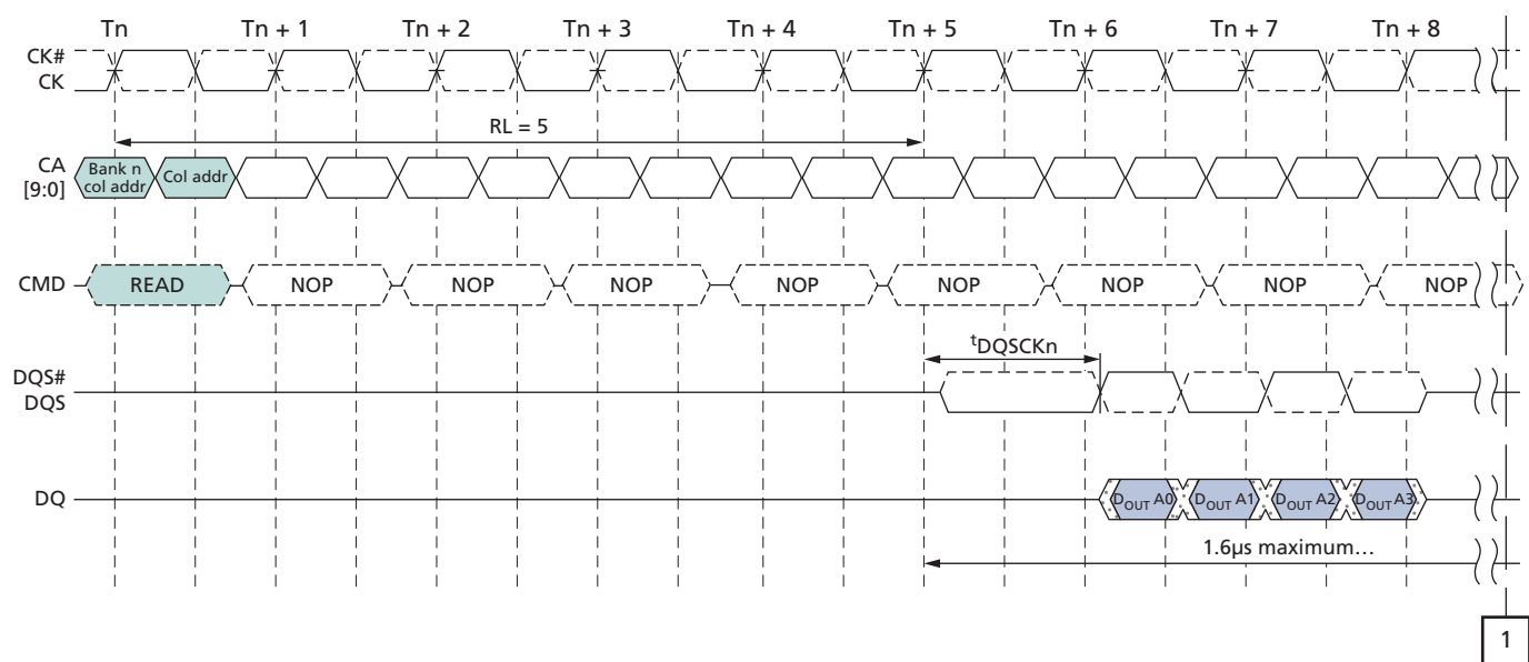
Figure 17: t_{DQSCDM} Timing
