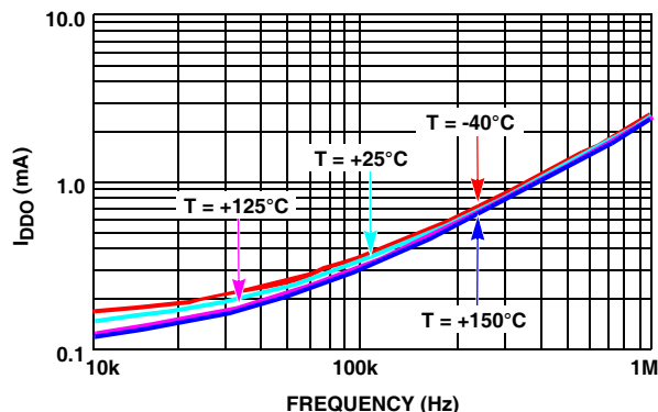
FIGURE 5. ISL89400 I DD OPERATING CURRENT vs FREQUENCY
