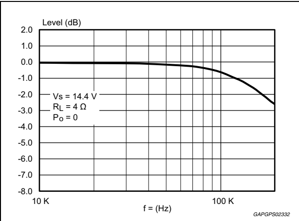
Figure 14. Power bandwidth
