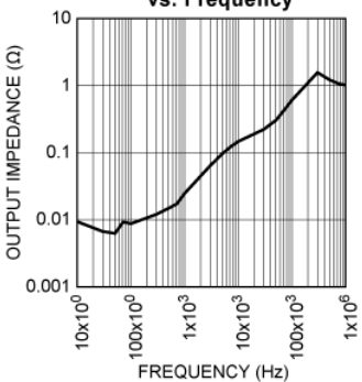
MIC2950x Output Impedance vs. Frequency
