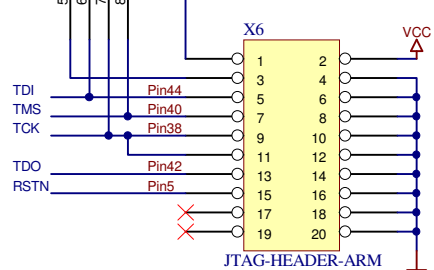
JTAG-Header for ARM
