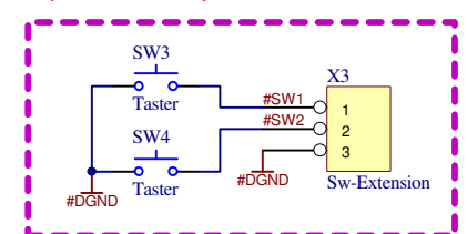
Separated PCB - only for case version
