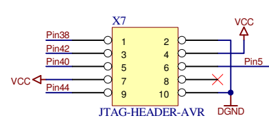
JTAG-Header for AVR
