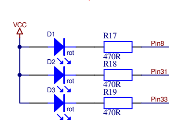
LEDs for User Output
