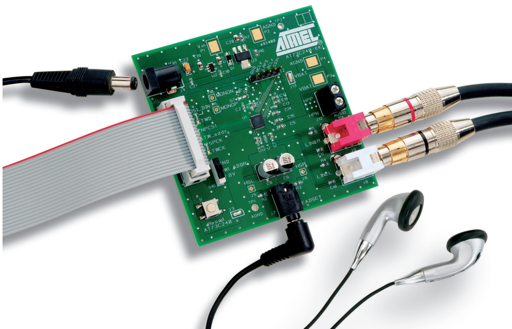
Figure 1-2. AT73C240-EK1Card With Available Connections
