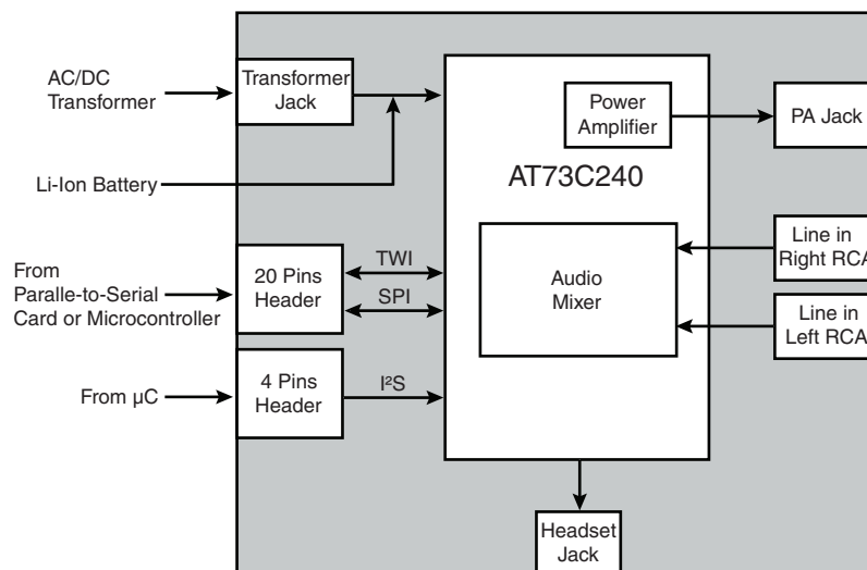
Figure 2-1. AT73C240-EK1 Block Diagram
