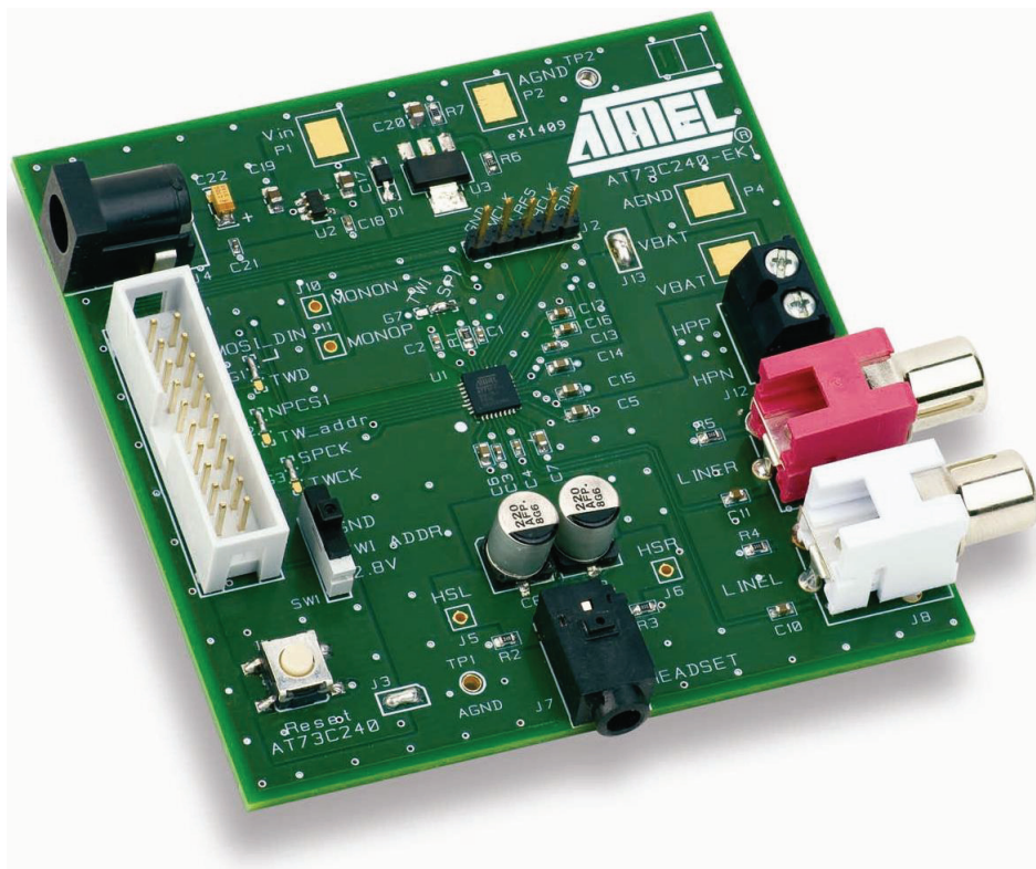
Figure 1-1. AT73C240-EK1 Top View (card photo)
