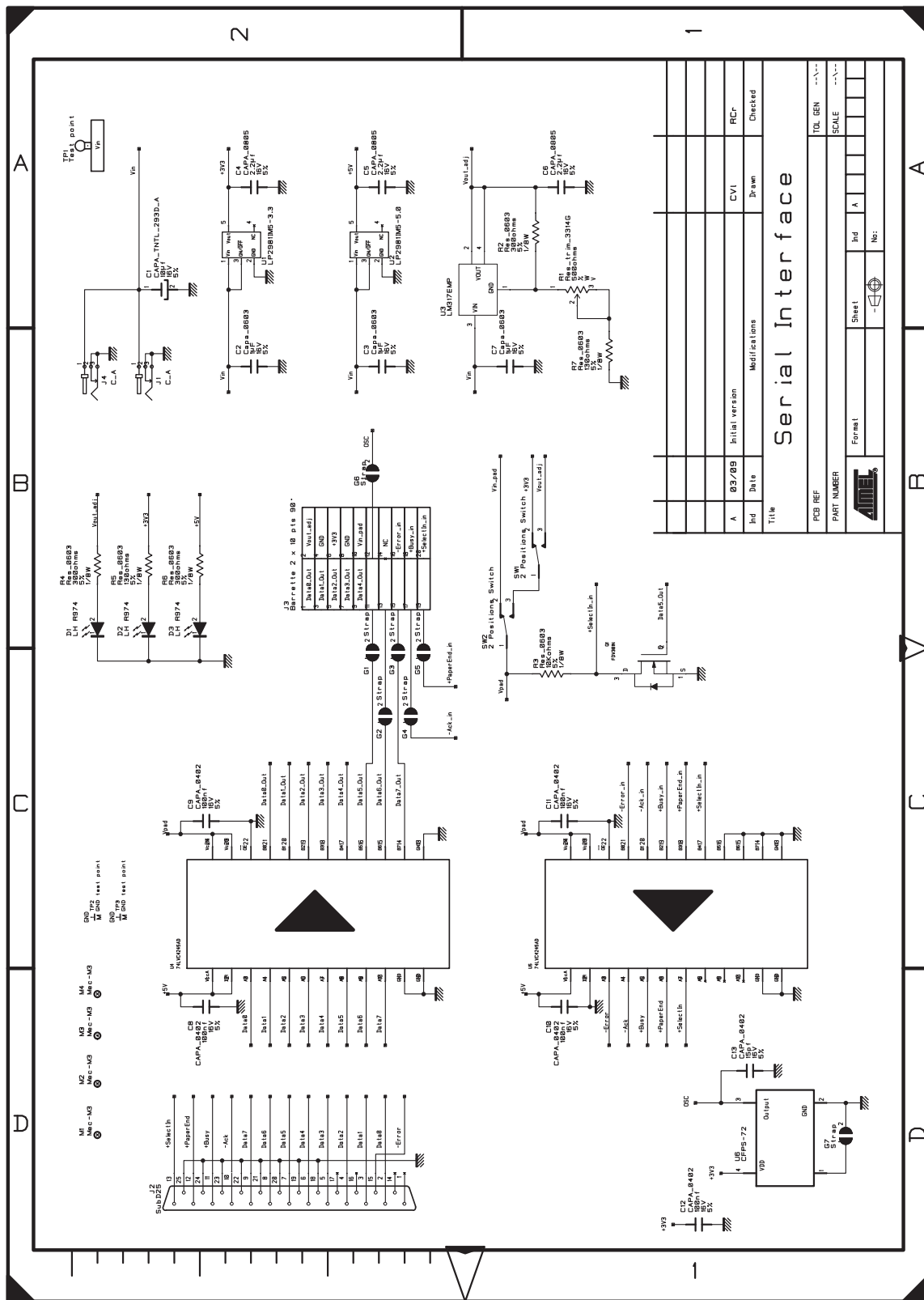
Figure 7-2. Parallel-to-Serial Card Schematic
