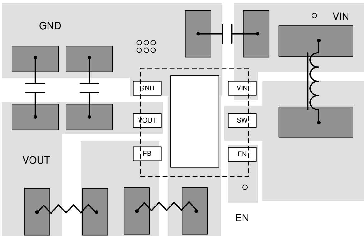
Figure 11-2. Layout - DRV
