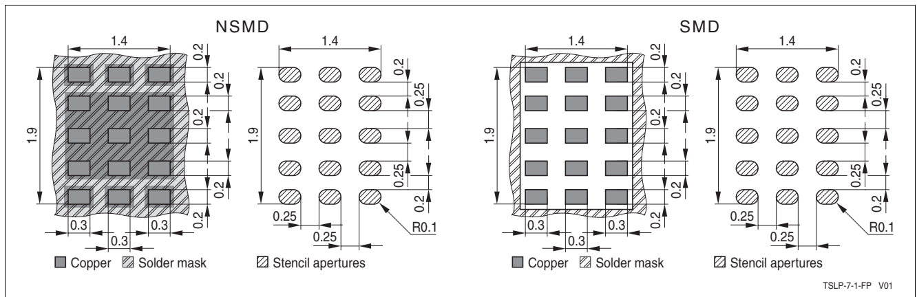
Figure 7 Recommended footprint and stencil layout for the TSLP-7-1 package
