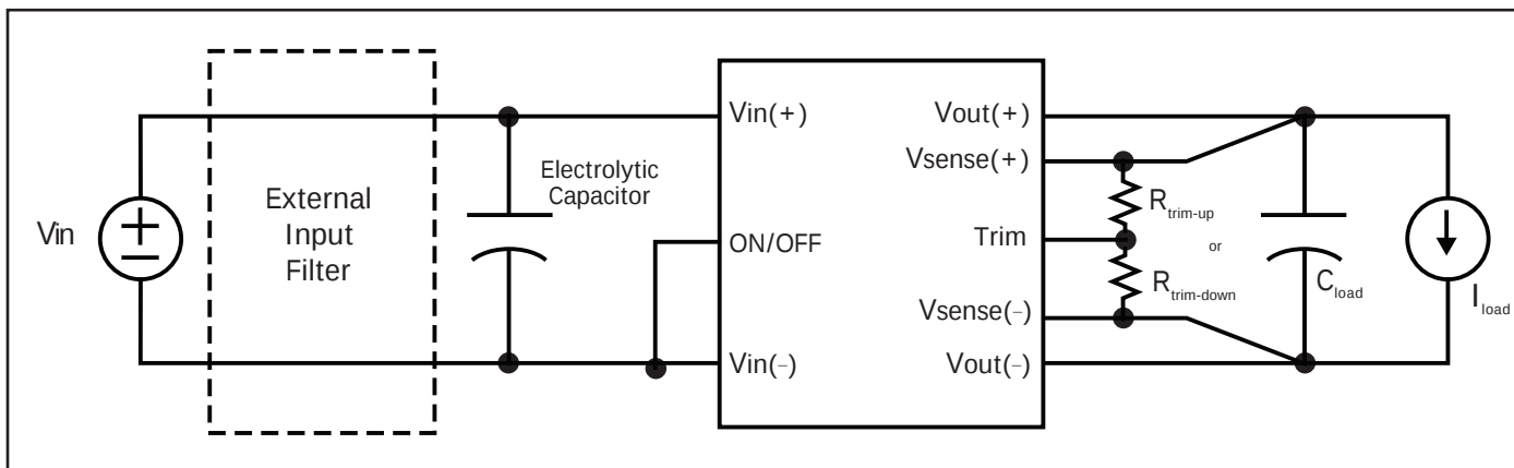
Figure D: Typical application circuit (negative logic unit, permanently enabled).
