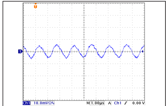
Figure 14: Input Terminal Ripple Current, i_c , at full rated output current and nominal input voltage with 10\mu H source impedance and 100\mu F electrolytic capacitor (Ch1 100mA/div). (See Figure 13).
