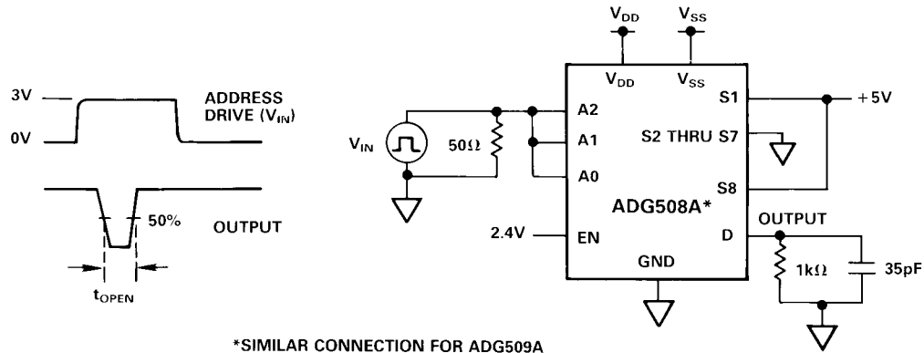
TEST CIRCUIT 7 BREAK-BEFORE-MAKE DELAY, t_{\text{OPEN}}
