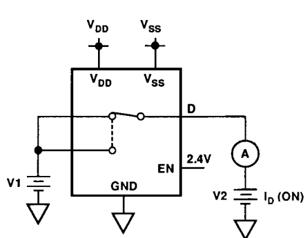
TEST CIRCUIT 4 I_D(\text{ON})
