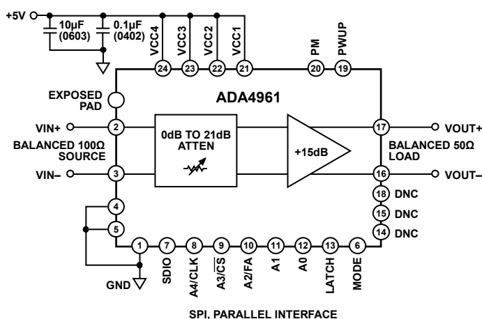
Figure 40. Basic Connections
