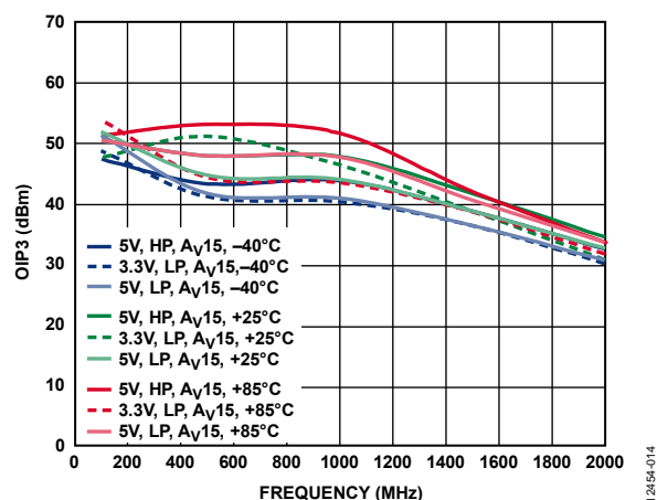
Figure 13. OIP3 vs. Frequency at Three Temperatures, Maximum Gain, 5.0 V, 3.3 V, with Low-Pass Filter
