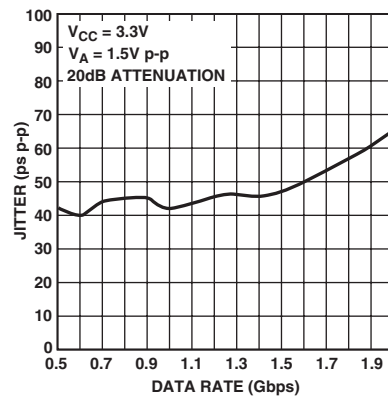
TPC 14. Jitter vs. Data Rate; PRBS 31
