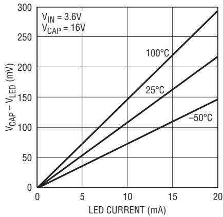
LED Pin Voltage Drop (V CAP - V LED )
