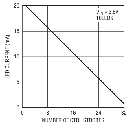
LED Current vs CTRL Strobe Pulses
