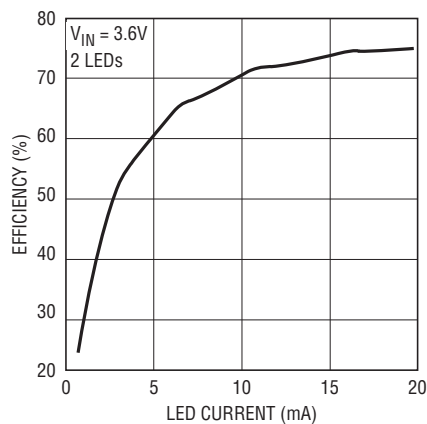
Conversion Efficiency
