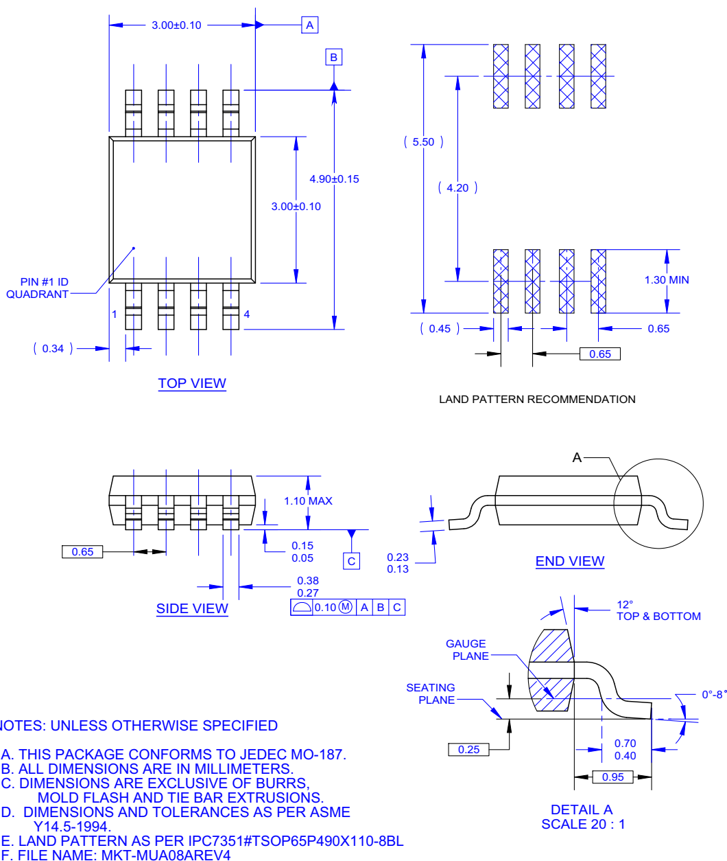
Figure 9. 8-LEAD, MSOP, JEDEC MO-187, 3.0MM WIDE
