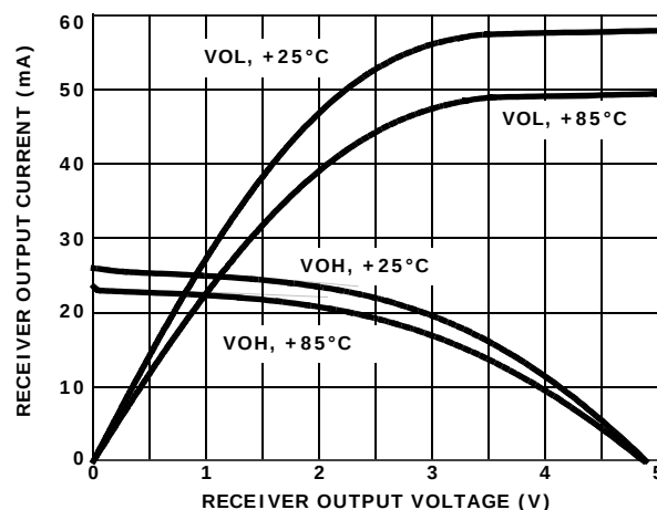
FIGURE 21. RECEIVER OUTPUT CURRENT vs RECEIVER OUTPUT VOLTAGE
