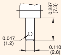
PCB Terminals – Straight 0.024 x 0.020 (0.6 x 0.5)
