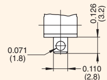
PCB Terminals RH Side w/o Location Pins 0.024 x 0.020 (0.6 x 0.5)
