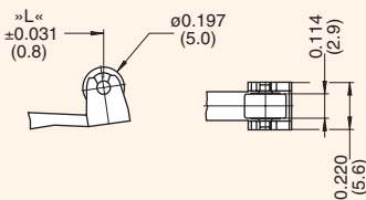
Simulated Roller – Plastic
