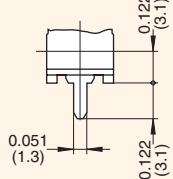
PCB Terminals LH Side w/o Location Pins 0.024 x 0.020 (0.6 x 0.5)
