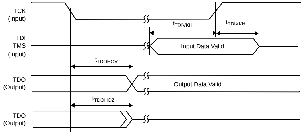
Figure 31. Test Access Port Timing
