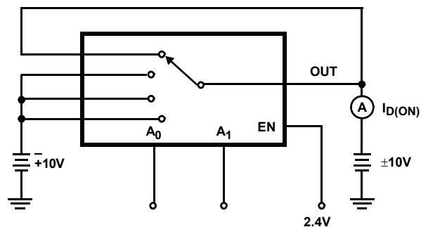
FIGURE 2D. I_{\text{D(ON)}} TEST CIRCUIT (NOTE 12)
