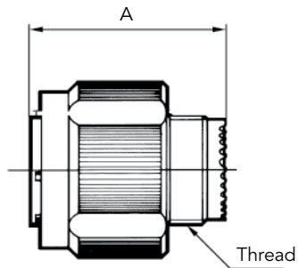
8D type 5 & D38999 type 26
