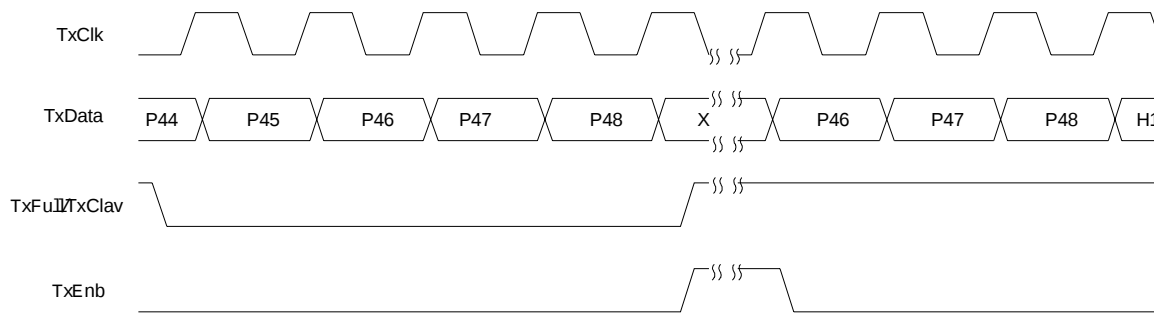
Figure 5 TxFull/TxClav Waveform
