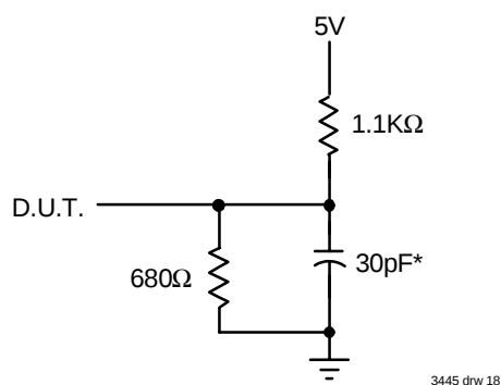
Figure 15 Output Load
