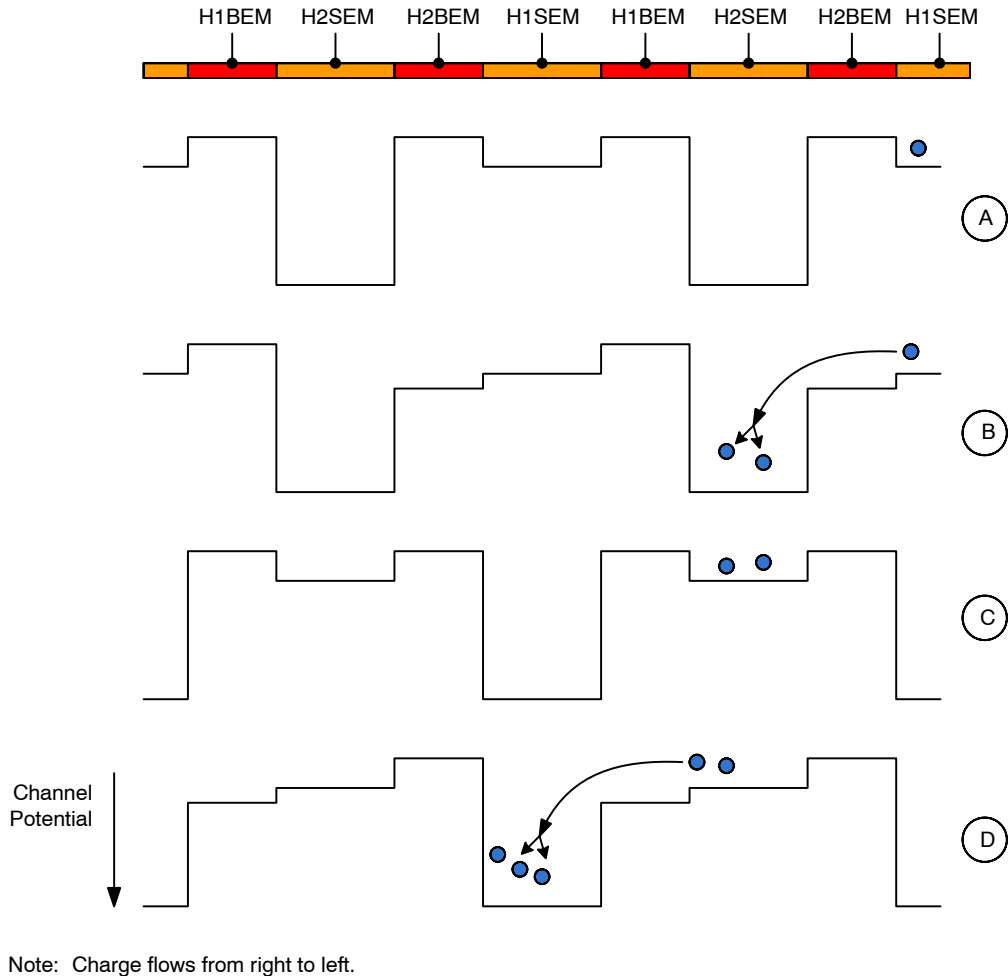
Figure 26. The Charge Multiplication Process
