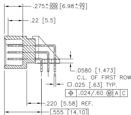
SECTION X-X
