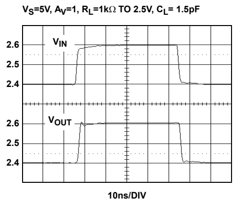
FIGURE 24. SMALL SIGNAL TRANSIENT RESPONSE
