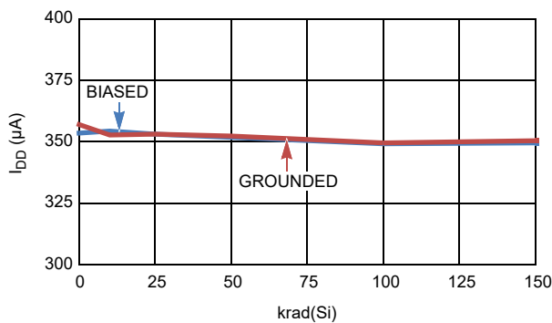
Figure 26. ISL7x6xEH I_{DD} vs Low Dose Rate Radiation
