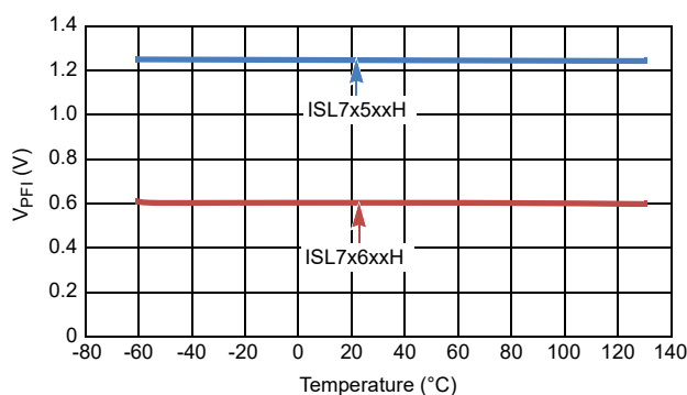
Figure 2. Precision Threshold Detector Temperature Characteristics Curve
