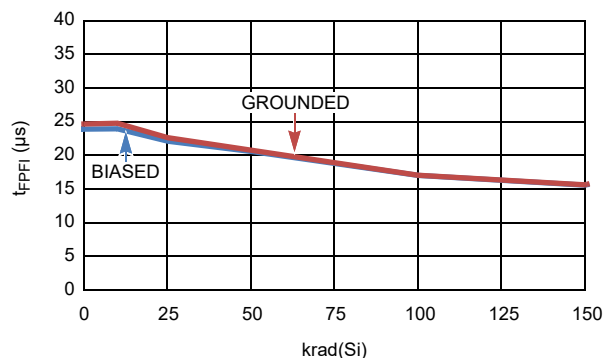
Figure 34. ISL7x6xEH t_{FPF1} vs Low Dose Rate Radiation
