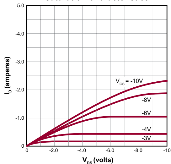
Saturation Characteristics
