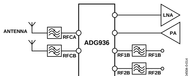
Figure 28. Tx/Rx Switching
