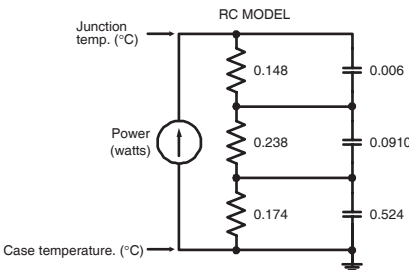
FIGURE 25b. TRANSIENT THERMAL IMPEDANCE MODEL
