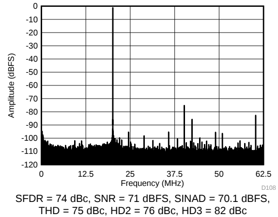
Figure 107. FFT for 270-MHz Input Signal (Dither Off)
