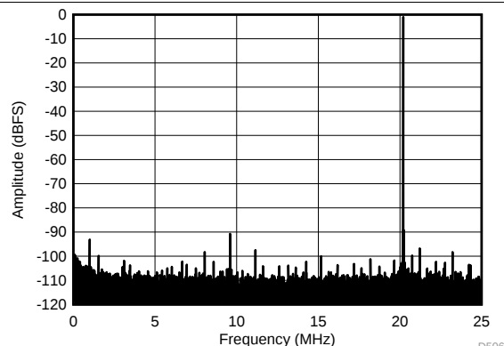
Figure 37. FFT for 70-MHz Input Signal (Dither Off)
