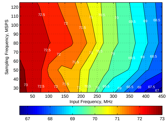
Figure 140. Signal-to-Noise Ratio (SNR)
