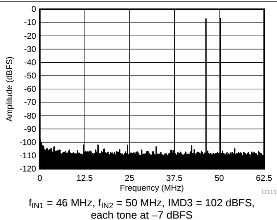
Figure 110. FFT for Two-Tone Input Signal ( -7\text{ dBFS} at 46 MHz and 50 MHz)
