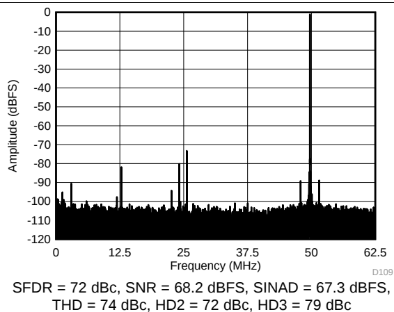
Figure 108. FFT for 450-MHz Input Signal (Dither On)
