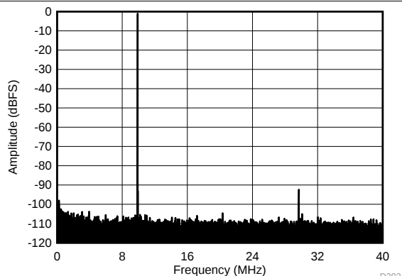
Figure 67. FFT for 10-MHz Input Signal (Chopper On, Dither On)
