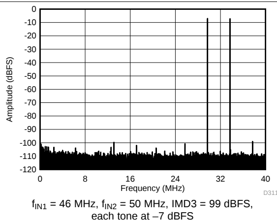
Figure 77. FFT for Two-Tone Input Signal ( -7\text{ dBFS} at 46 MHz and 50 MHz)
