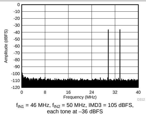
Figure 78. FFT for Two-Tone Input Signal ( -36\text{ dBFS} at 46 MHz and 50 MHz)
