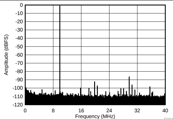
Figure 68. FFT for 10-MHz Input Signal (Chopper On, Dither Off)
