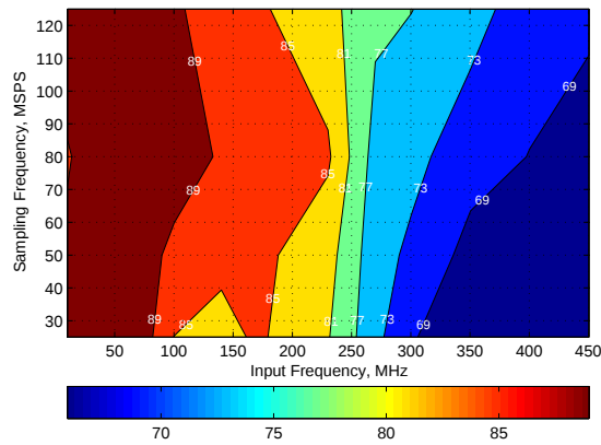
Figure 139. Spurious-Free Dynamic Range (SFDR)
