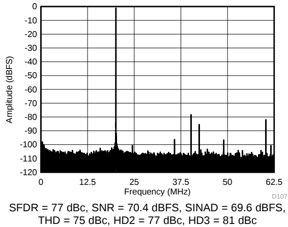
Figure 106. FFT for 270-MHz Input Signal (Dither On)
