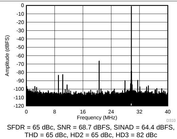
Figure 76. FFT for 450-MHz Input Signal (Dither Off)
