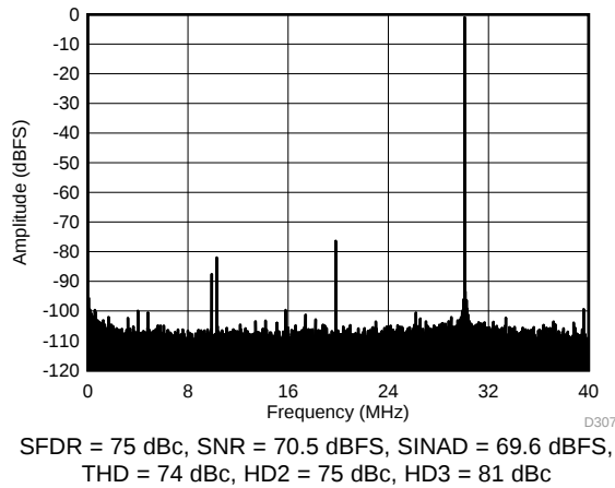
Figure 73. FFT for 270-MHz Input Signal (Dither On)
