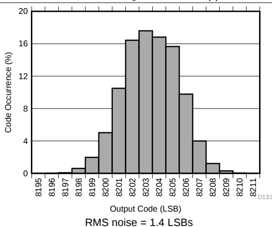
Figure 130. Idle Channel Histogram
