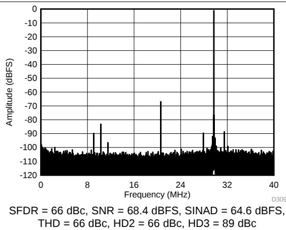
Figure 75. FFT for 450-MHz Input Signal (Dither On)
