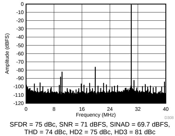
Figure 74. FFT for 270-MHz Input Signal (Dither Off)
