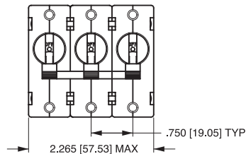
3-POLE (BA3)
