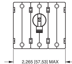
3-POLE (BB3)
