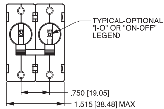
2-POLE (BA2)
