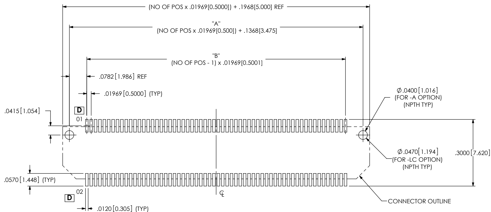
FIG 1 BTH-060-XX-X-D-XX SHOWN
