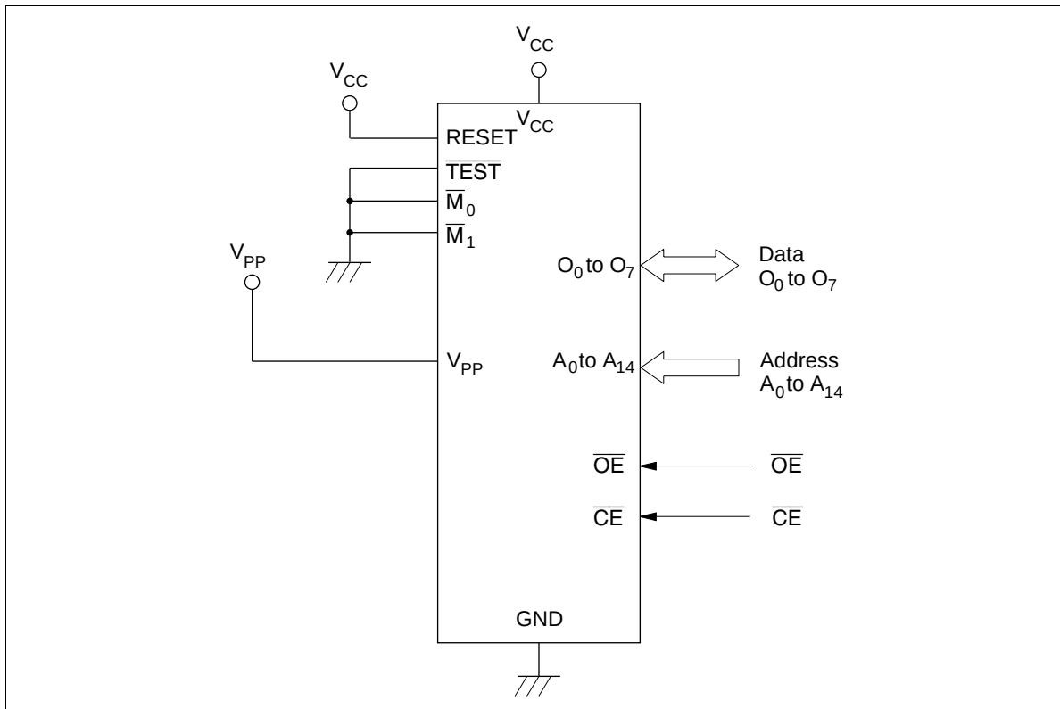
Figure 38 PROM Mode Function Diagram
