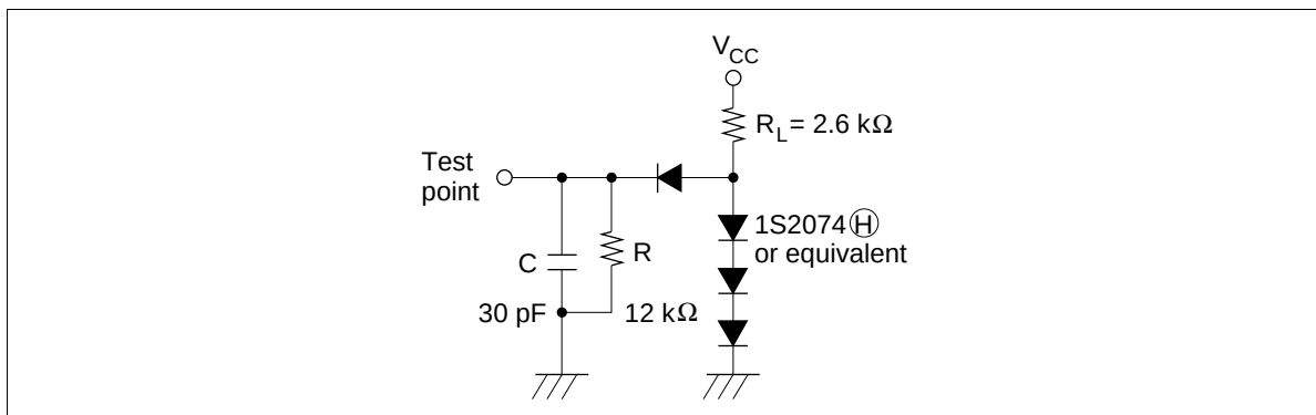
Figure 52 Timing Load Circuit
