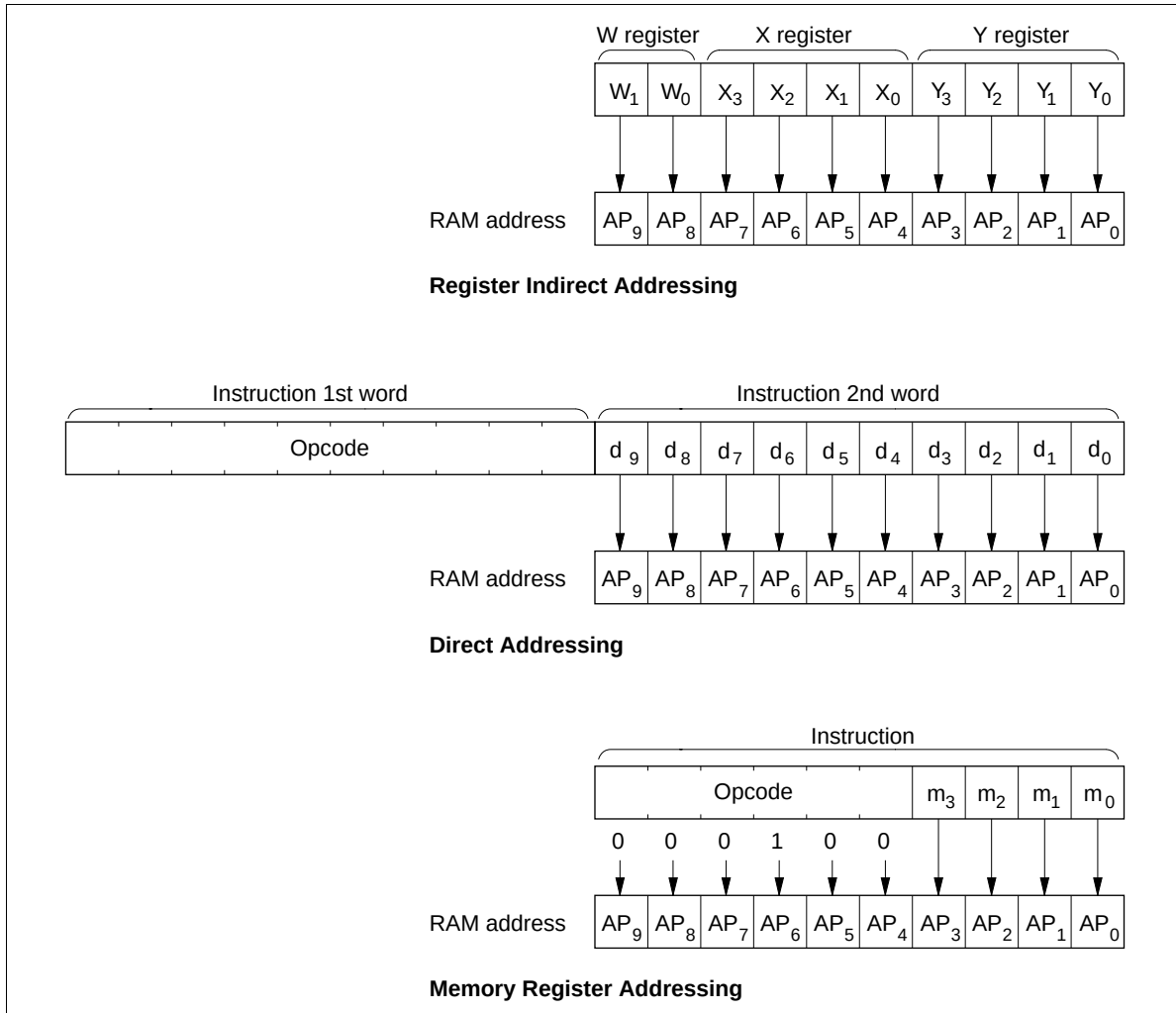
Figure 39 RAM Addressing Modes
