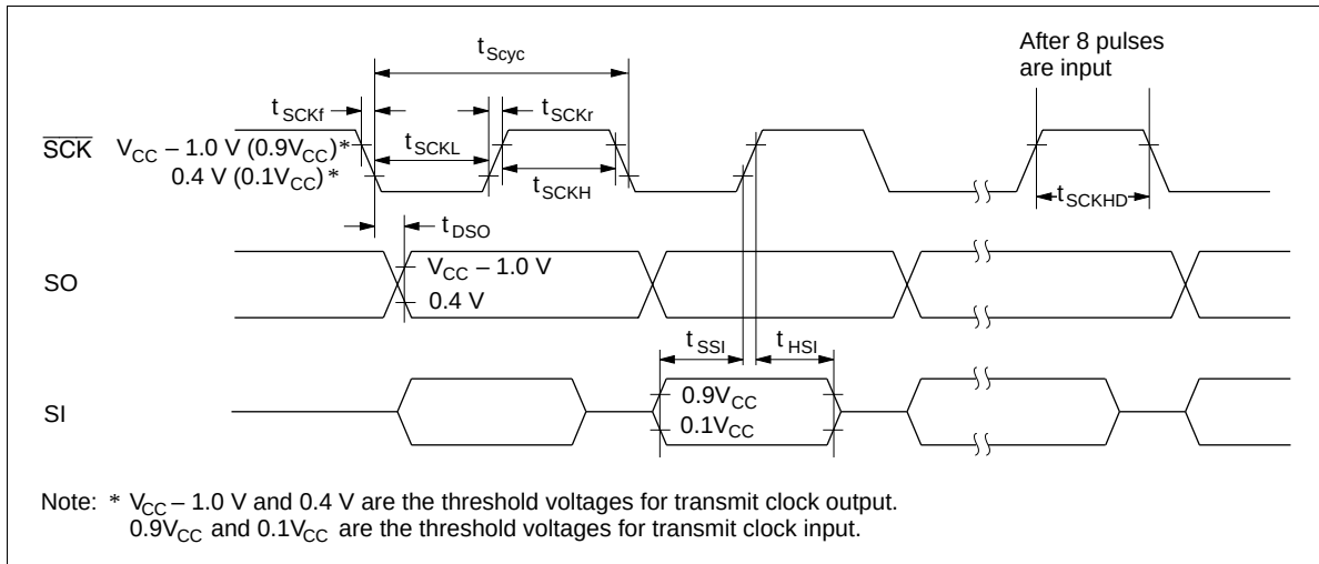
Figure 51 Timing of Serial Interface
