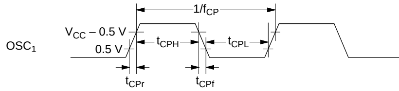
Figure 43 Oscillator Timing
