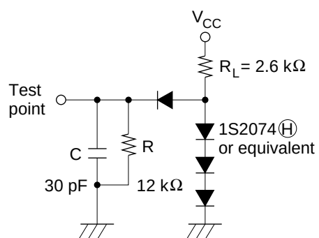
Figure 47 Timing Load Circuit
