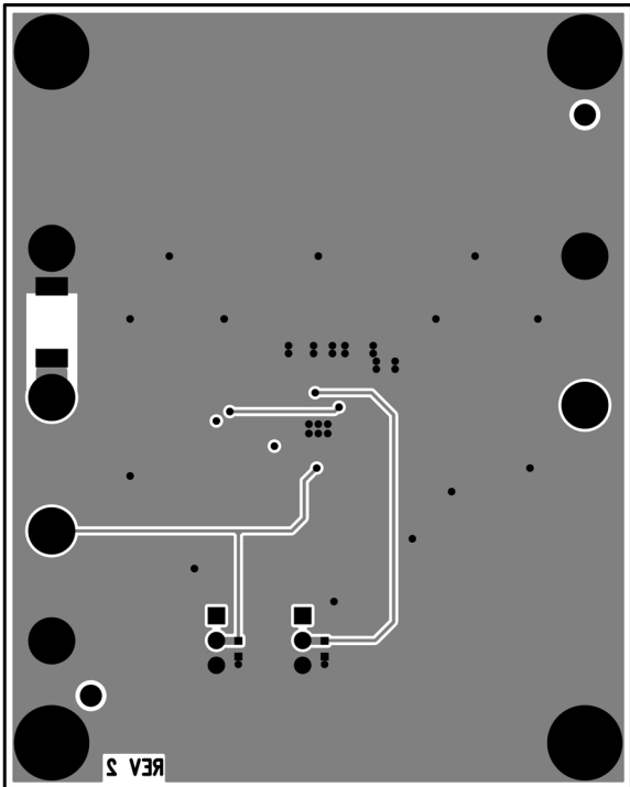
Figure 17c. Bottom Layer of Example PCB
