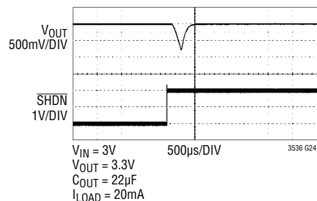
Start-Up in PWM Mode Operation with Output Precharged
