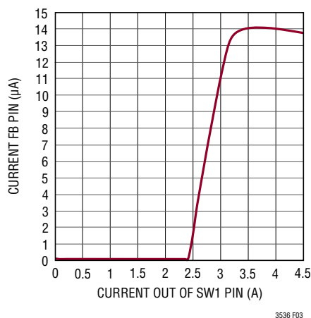
Figure 3. FB Current for Input Current Limitation
