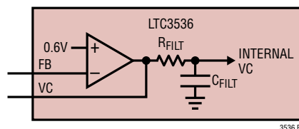
Figure 9. Internal Loop Filter
