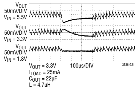
Burst Mode Operation to PWM Mode Transient
