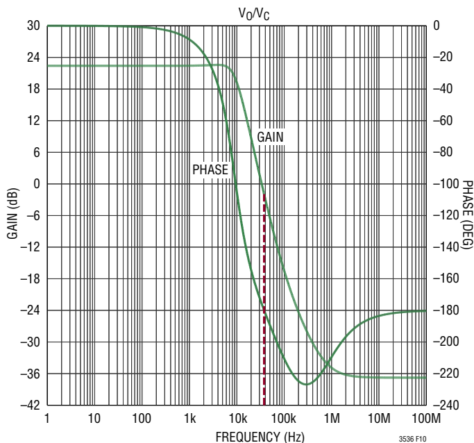
Figure 10. Converter Bode Plot, V_{IN} = 1.8\text{V} , I_{LOAD} = 300\text{mA}
