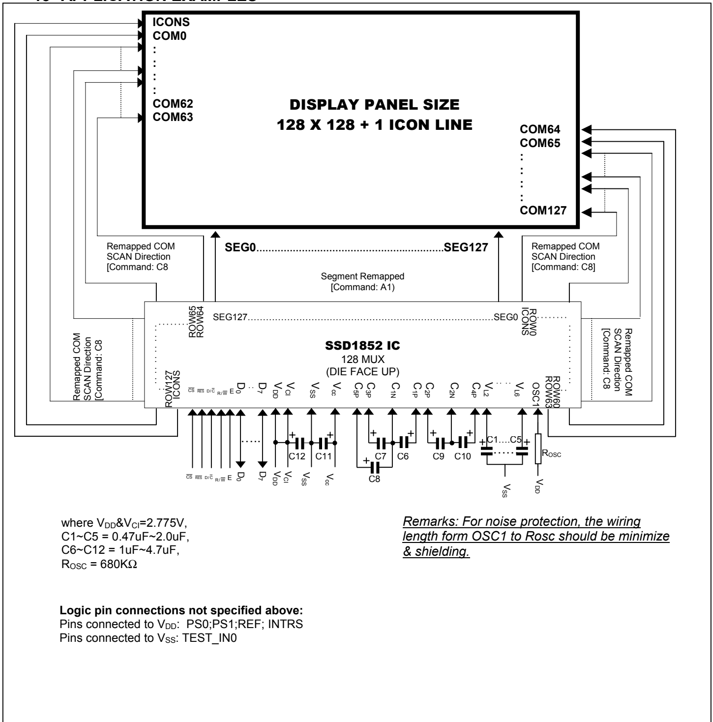
Figure 19 - Typical Application
