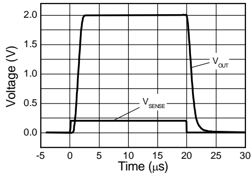
Forward Large Signal Step Response
