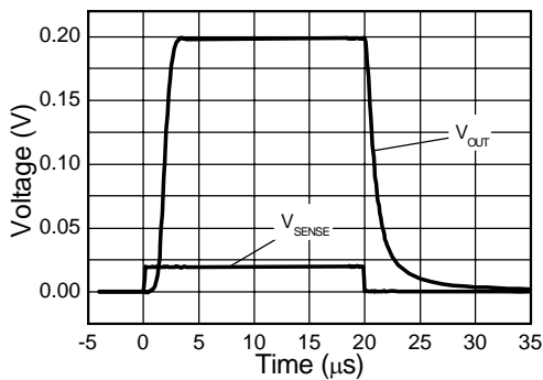
Forward Small Signal Step Response
