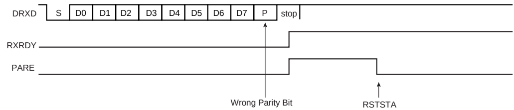
Figure 26-8. Parity Error
