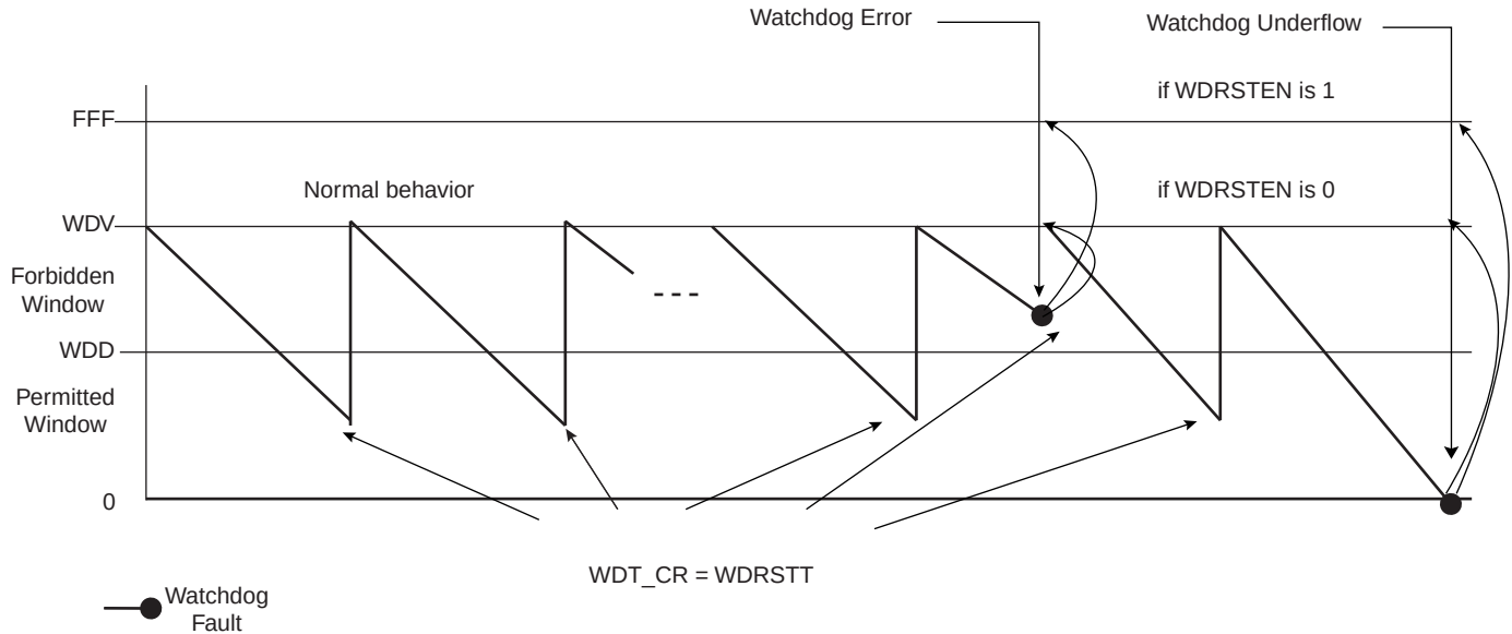
Figure 16-2. Watchdog Behavior
