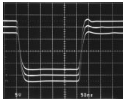
R_F = 750\Omega R_L = 10\Omega I_Q = 9\text{mA}, 18\text{mA}, 36\text{mA} V_S = \pm 15\text{V}
