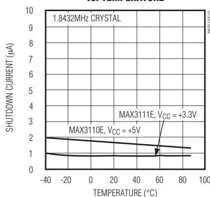
UART SHUTDOWN CURRENT vs. TEMPERATURE
