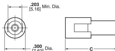
Plug
