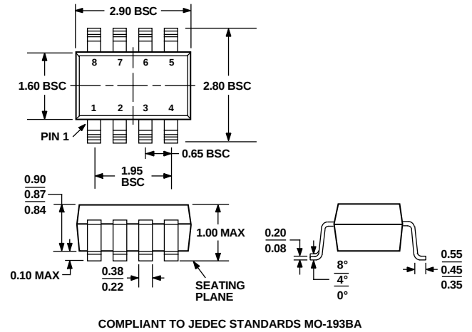
Figure 36. 8-Lead Thin Small Outline Transistor Package [TSOT] (UJ-8)
