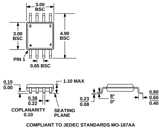
Figure 35. 8-Lead Mini Small Outline Package [MSOP] (RM-8)
