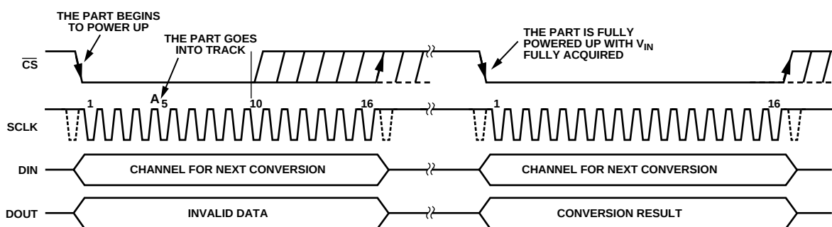
Figure 28. Exiting Power-Down Mode
