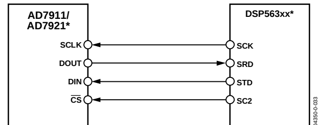
Figure 34. Interfacing to the DSP563xx
