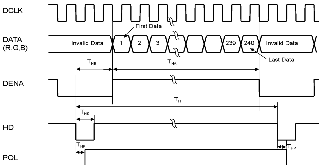
b. Horizontal Timing Chart
