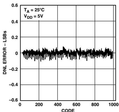
Figure 9. AD5333 Typical DNL Plot
