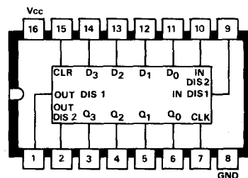
B120 SN74173N SN74C173N Quad D Bus flip-flop
