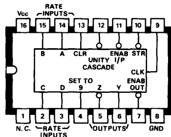
B118 SN74167N SN74C167N Decade rate multiplier
