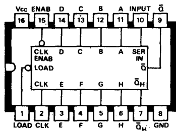
B116 SN74165N SN74L165N/SN74C165N 8-bit shift register
