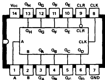
B115 SN74164N SN74C164N 8-bit shift register
