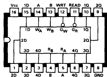
B119 SN74170N SN74S170N 4 by 4 bit shift register
