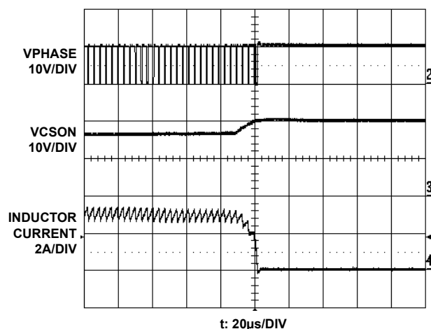
FIGURE 11. BATTERY REMOVAL
