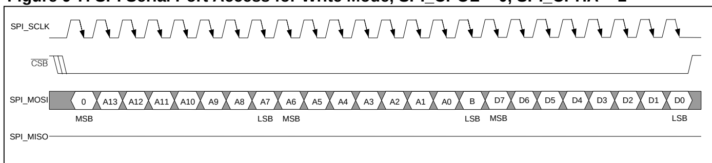
Figure 9-7. SPI Serial Port Access for Write Mode, SPI_CPOL = 0, SPI_CPHA = 1
