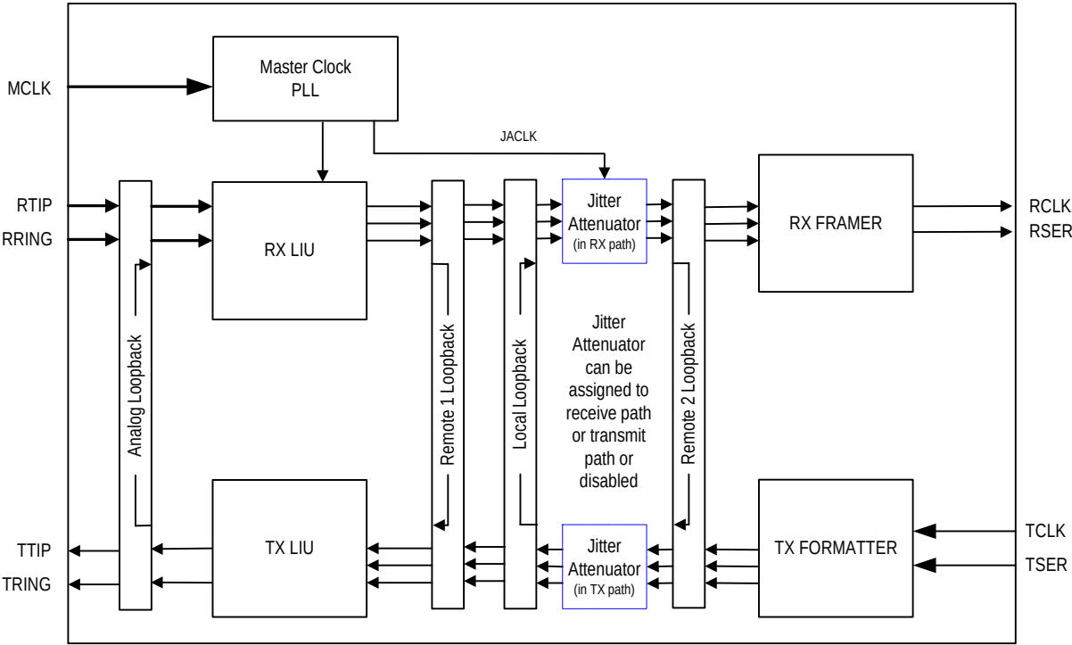
Figure 9-27. Loopback Diagram
