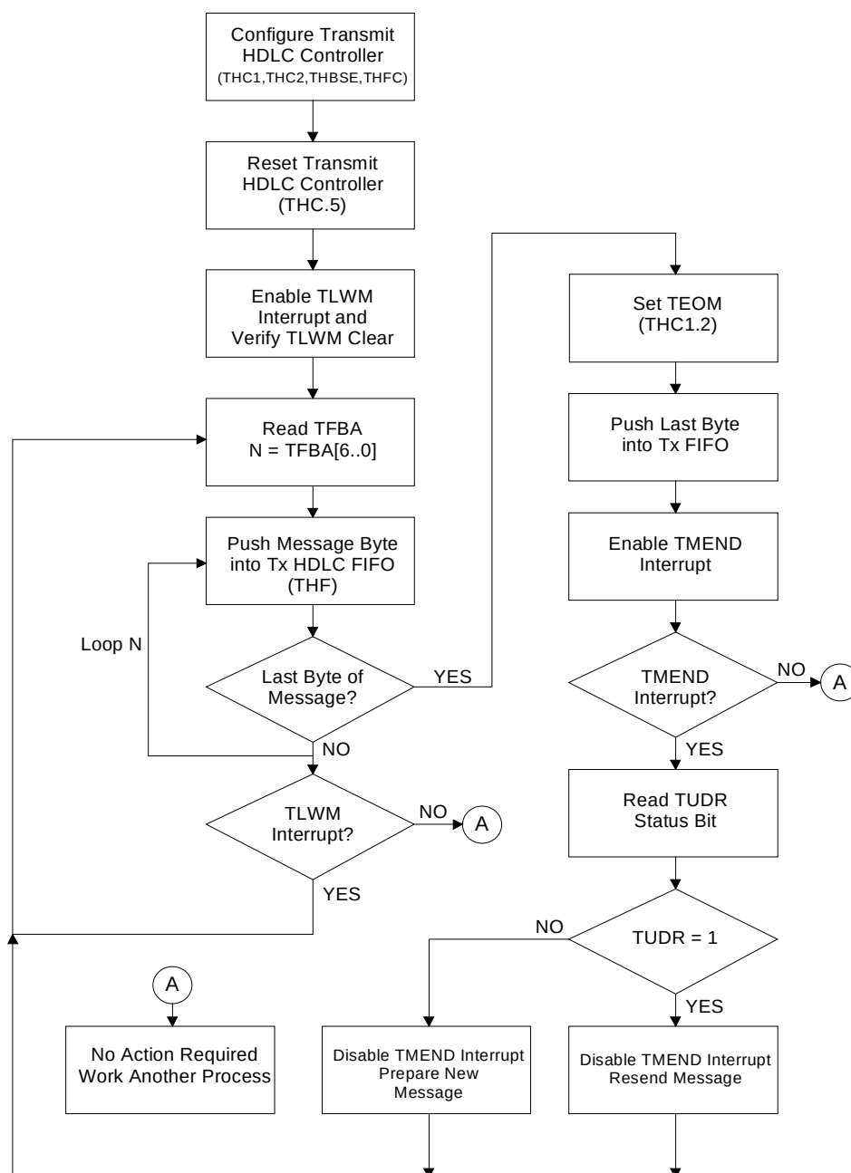
Figure 9-19. HDLC Message Transmit Example
