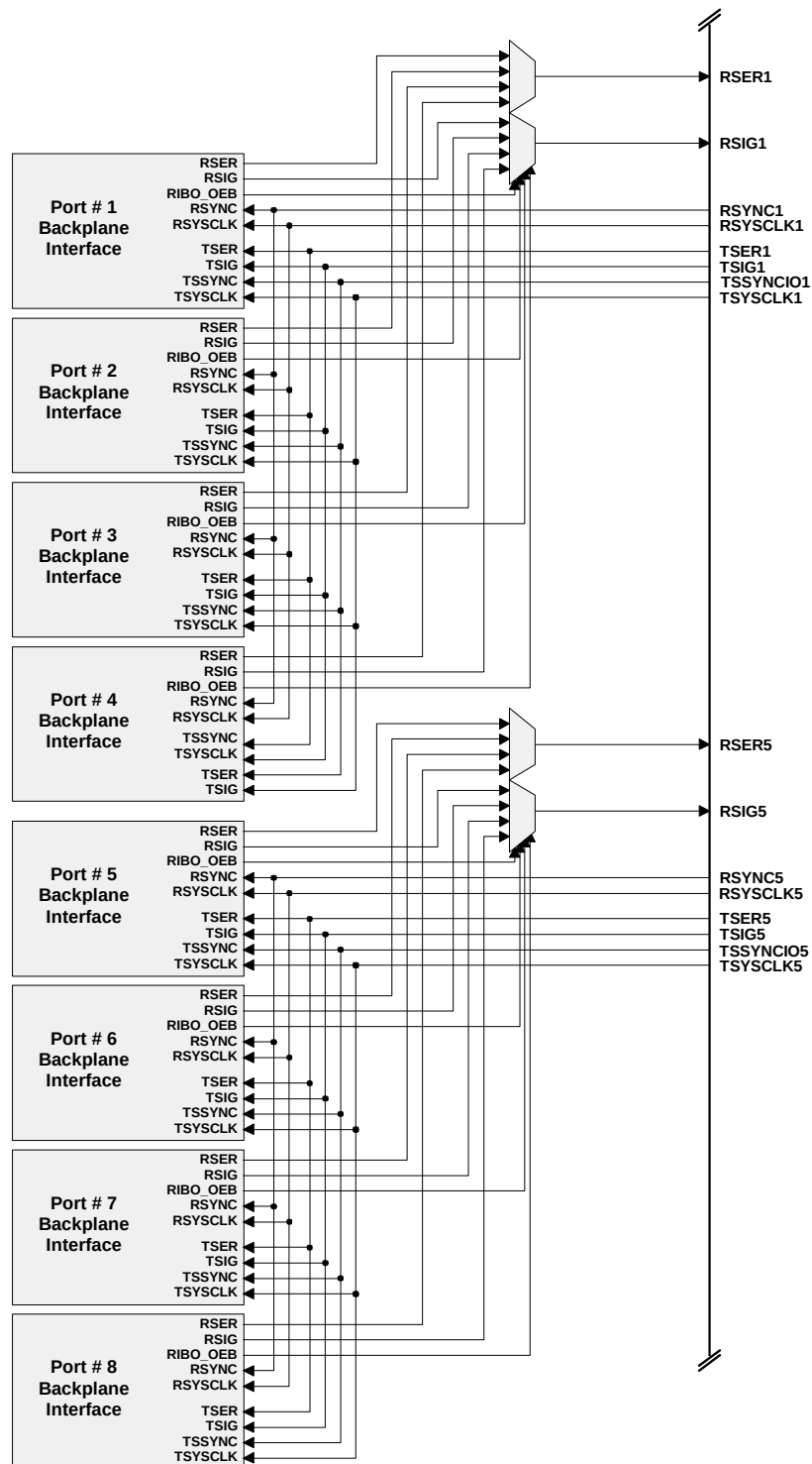
Figure 9-13. IBO Multiplexer Equivalent Circuit—8.192MHz
