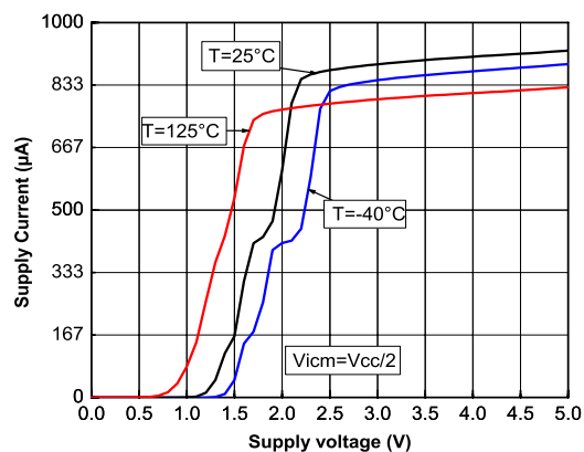
Figure 15. Supply current vs. supply voltage
